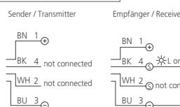
4-polig / 4-pin pnp
