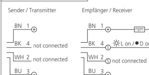
4-polig / 4-pin npn
